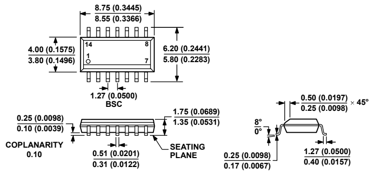
Figure 44. 14-Lead Standard Small Outline Package [SOIC_N] Narrow Body (R-14) Dimensions shown in millimeters and (inches)
