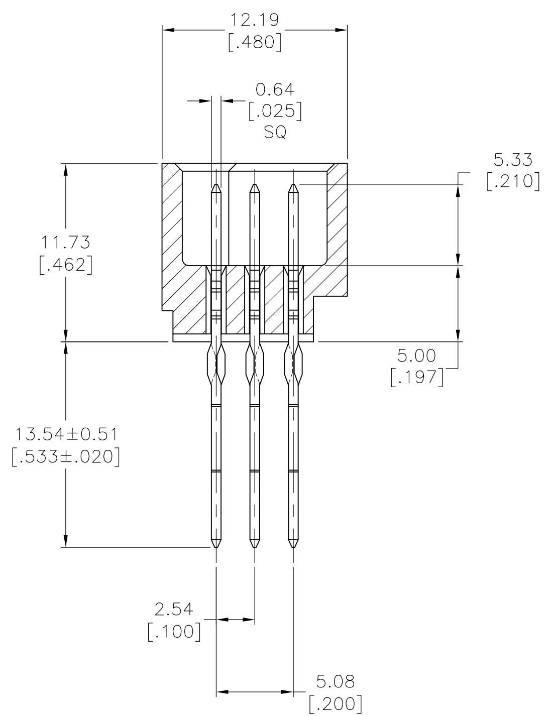
SECTION T-T
