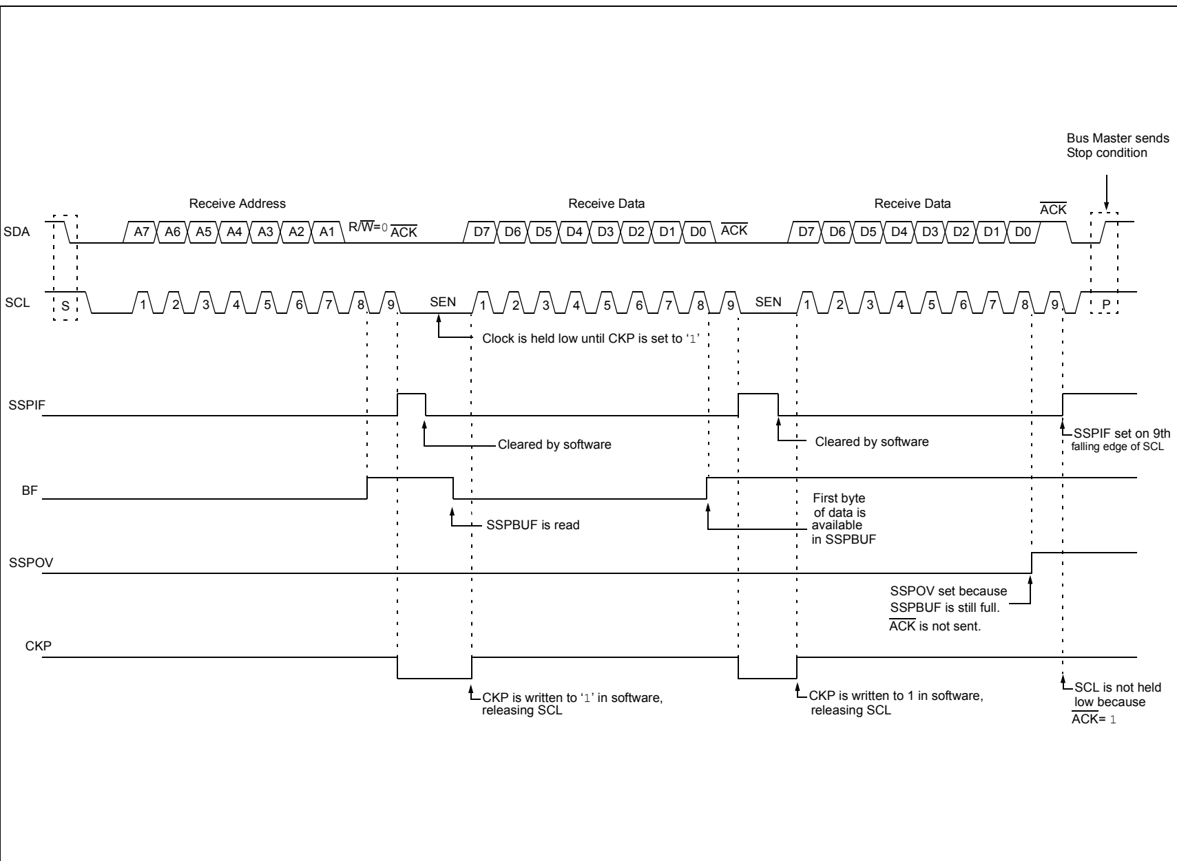
12C SLAVE, 7-BIT ADDRESS, RECEPTION (SEN = 1, AHEN = 0, DHEN = 0)
