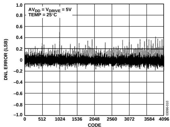
Figure 10. Typical DNL
