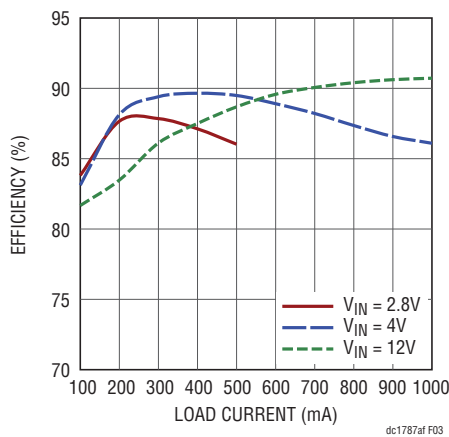
Figure 3. Efficiency Curves
