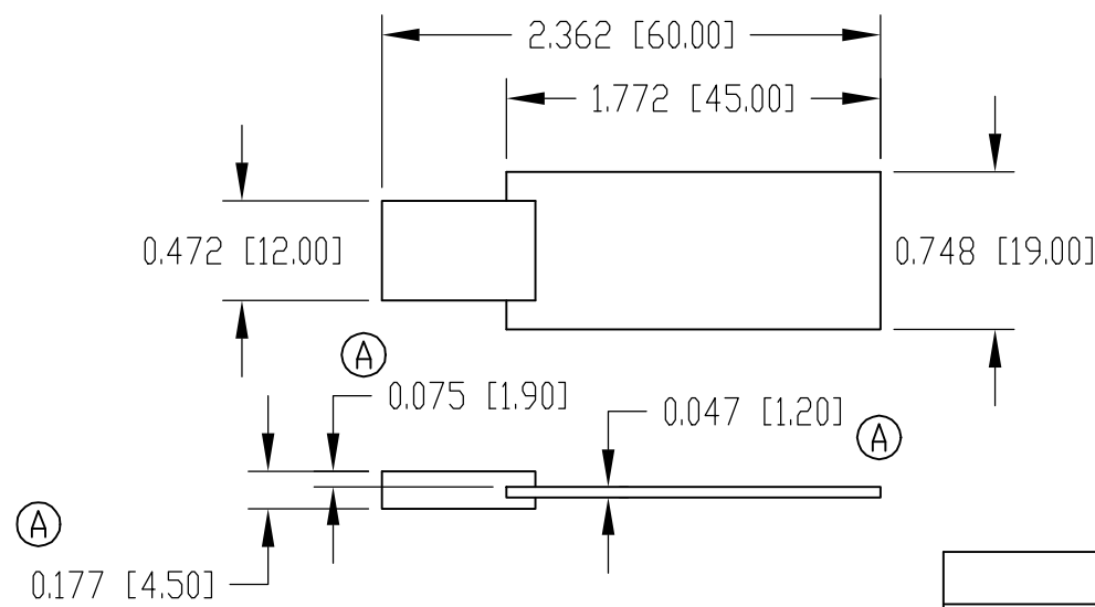
RECOMMENDED PCB SIZE
