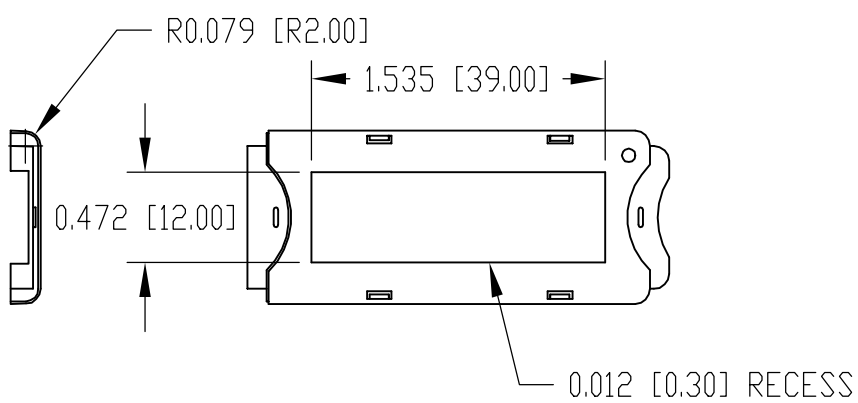
BASE
