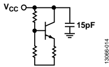
Figure 5. V CC Interface
