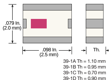
Case 39-1 (2520)
