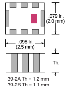
Case 39-2 (2520)
