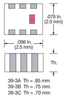
Case 39-3 (2520)
