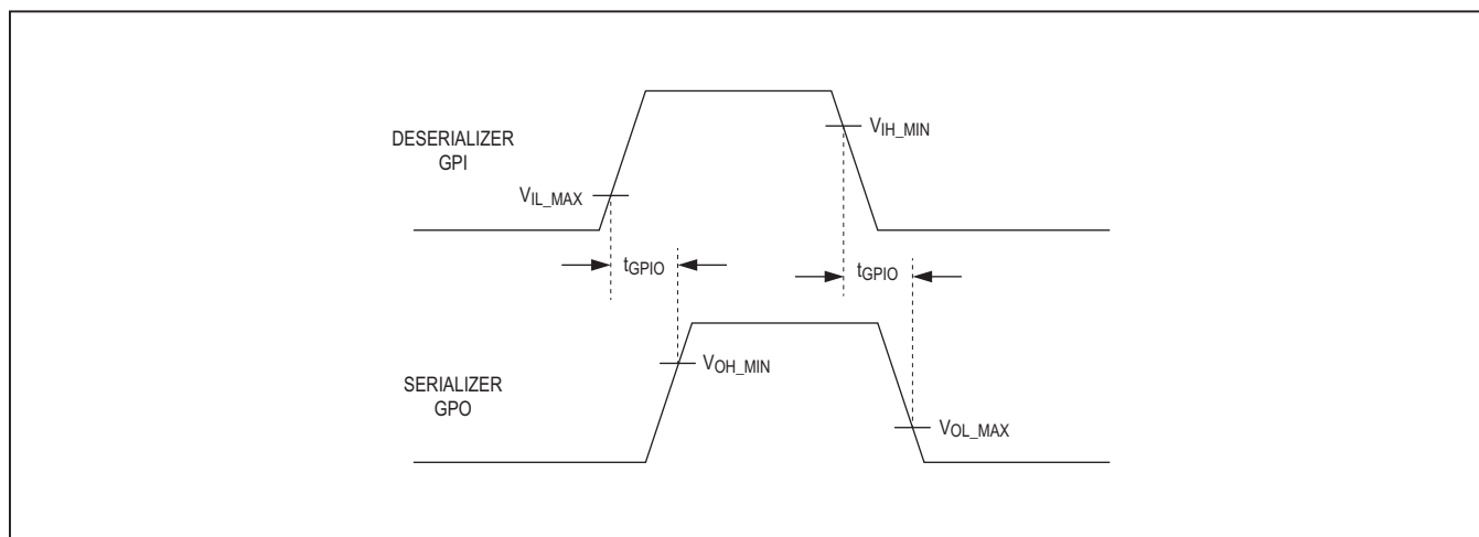
Figure 12. GPI-to-GPO Delay
