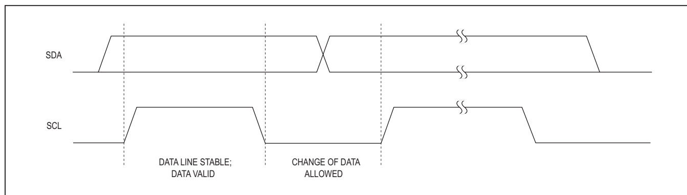
Figure 34. Bit Transfer
