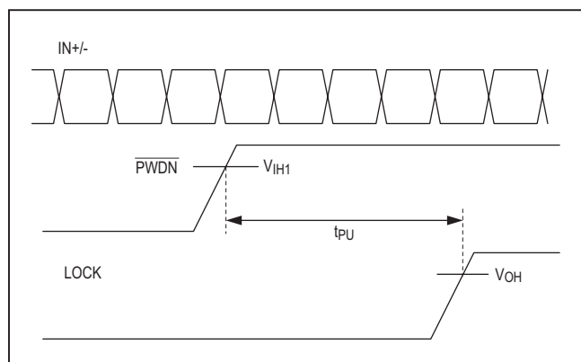
Figure 14. Power-Up Delay
