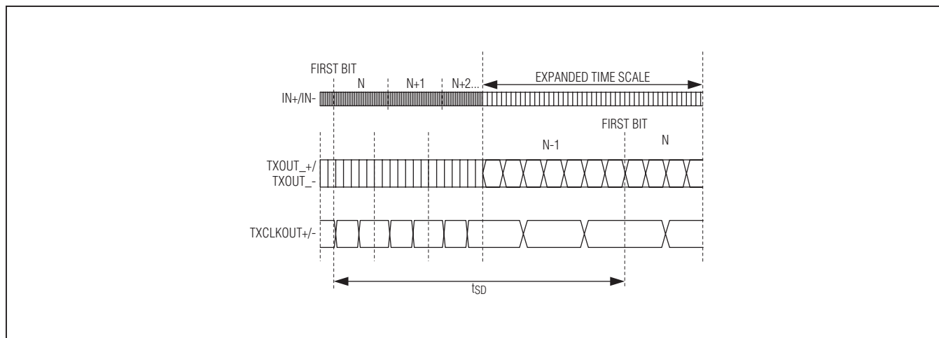
Figure 11. Deserializer Delay
