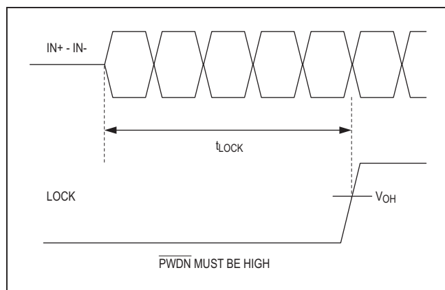
Figure 13. Lock Time
