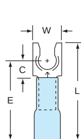
MH14-10FL Stud Size 10 Wire Range 16-14
