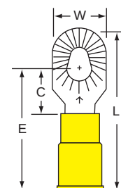
13-610-NB Stud Size Wire Range 6, 8, 10 12-10
