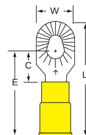
13-610-P Stud Size Wire Range 6, 8, 10 12-10
