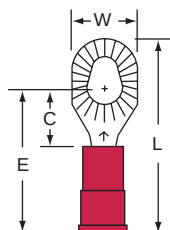
11-610-P Stud Size Wire Range 6, 8, 10 22-18
