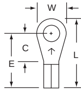
12-8S Stud Size 8 Wire Range 16-14
