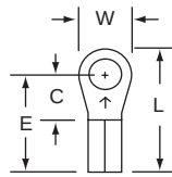
12-6S Stud Size 6 Wire Range 16-14
