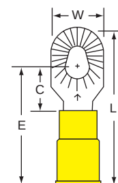
13-610-NB Stud Size 6, 8, 10 Wire Range 12-10
