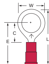
11-38-P Stud Size 3/8 Wire Range 22-18
