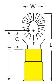
13-610-P Stud Size 6, 8, 10 Wire Range 12-10
