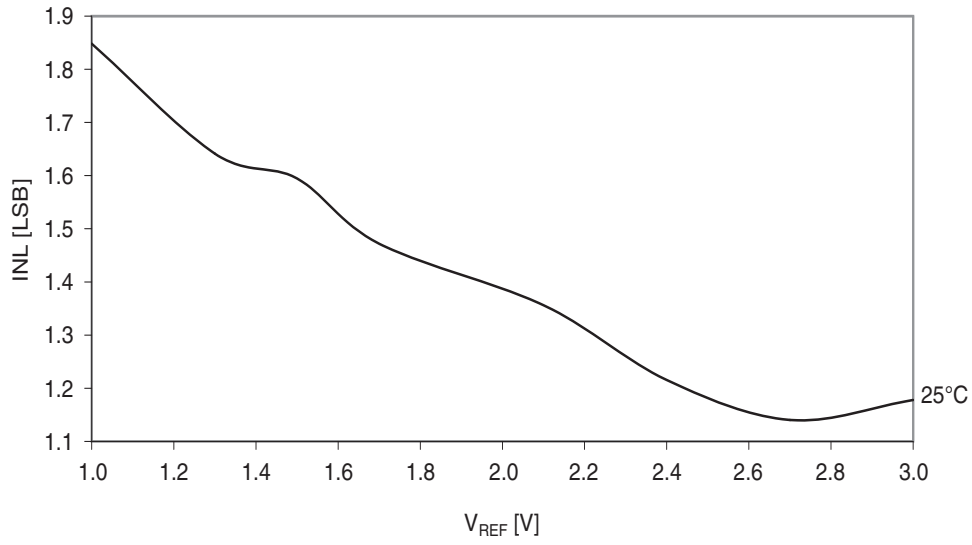
Figure 37-301. DAC INL error vs. V_{REF} V_{CC} = 3.6V
