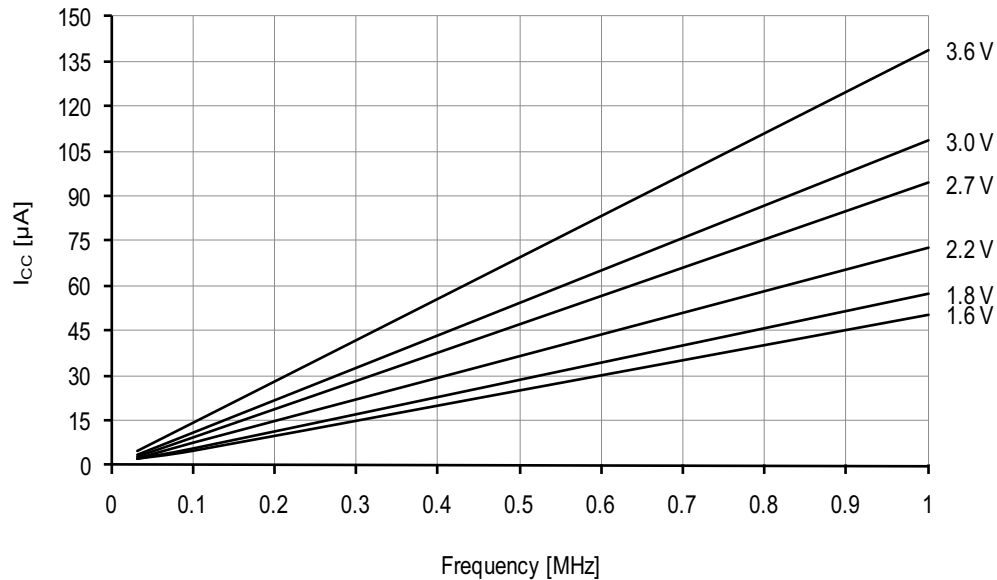
Figure 37-176. Idle mode supply current vs. frequency.
