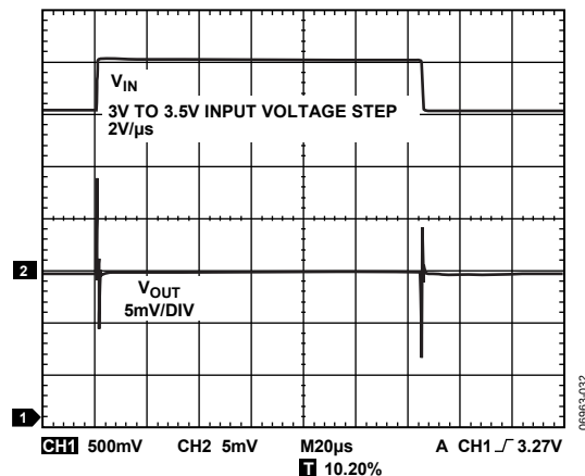
Figure 32. V_{IN} Line Transient Response, V_{BIAS} = 5\text{ V} , I_{OUT} = 350\text{ mA}
