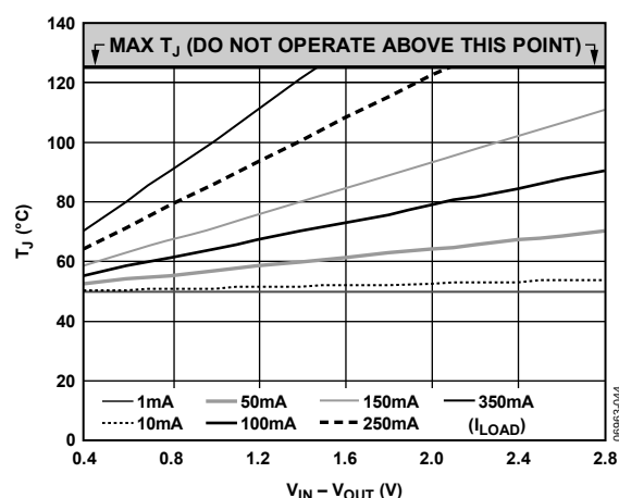
Figure 44. 100 \text{mm}^2 of PCB Copper, T_A = 50^{\circ}\text{C} , TSOT
