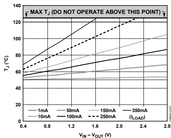
Figure 43. 500 \text{mm}^2 of PCB Copper, T_A = 50^{\circ}\text{C} , TSOT
