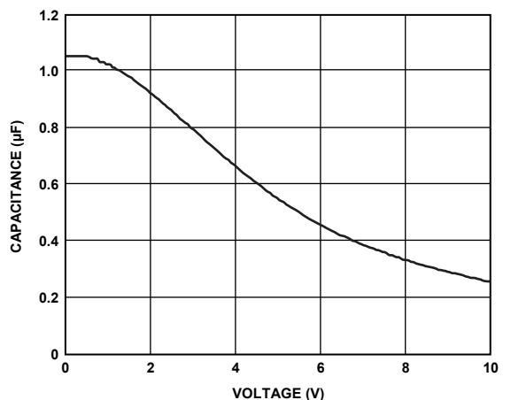
Figure 36. Capacitance vs. Voltage Characteristics
