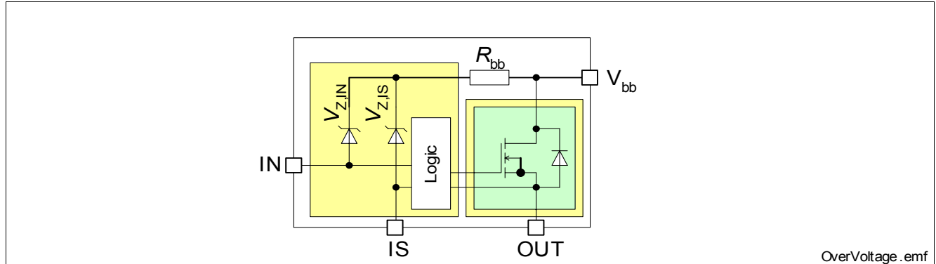
Figure 15 Overvoltage Protection
