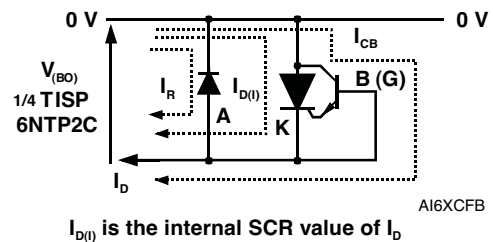
Figure 5. Off-State Current Verification
