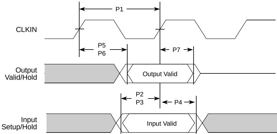
Figure 13. PCI Timing
