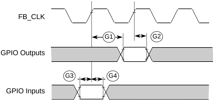
Figure 26. GPIO Timing
