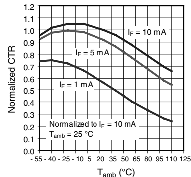
Fig. 9 - CTR Normalized to I_F = 10\text{ mA} vs. Ambient Temperature, (Non-Saturated, V_{CE} = 5\text{ V} )
