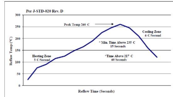
Figure 48. Recommended linear reflow profile using Sn/Ag/Cu solder.
