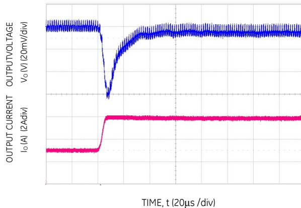
Figure 28. Transient Response to Dynamic Load Change from 50% to 100% at 12V in , C out -3x47μF, C Tune -178 & R Tune -3900pF
