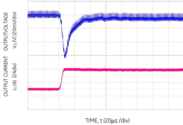
Figure 28. Transient Response to Dynamic Load Change from 50% to 100% at 12Vin, Cout-3x47uF, CTune-178 & RTune-3900pF
