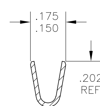
SECT B-B
