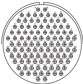
Insert Arrangement 44-52 Service Rating A Number of Contacts 104 Contact Size 16
