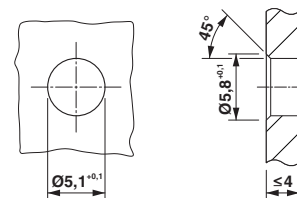
Dimensioned drawing
