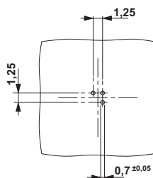
M5 flush-type plug
