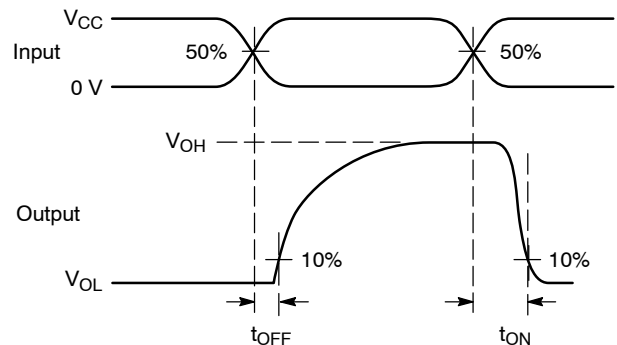
Figure 6. t_{ON}/t_{OFF}
