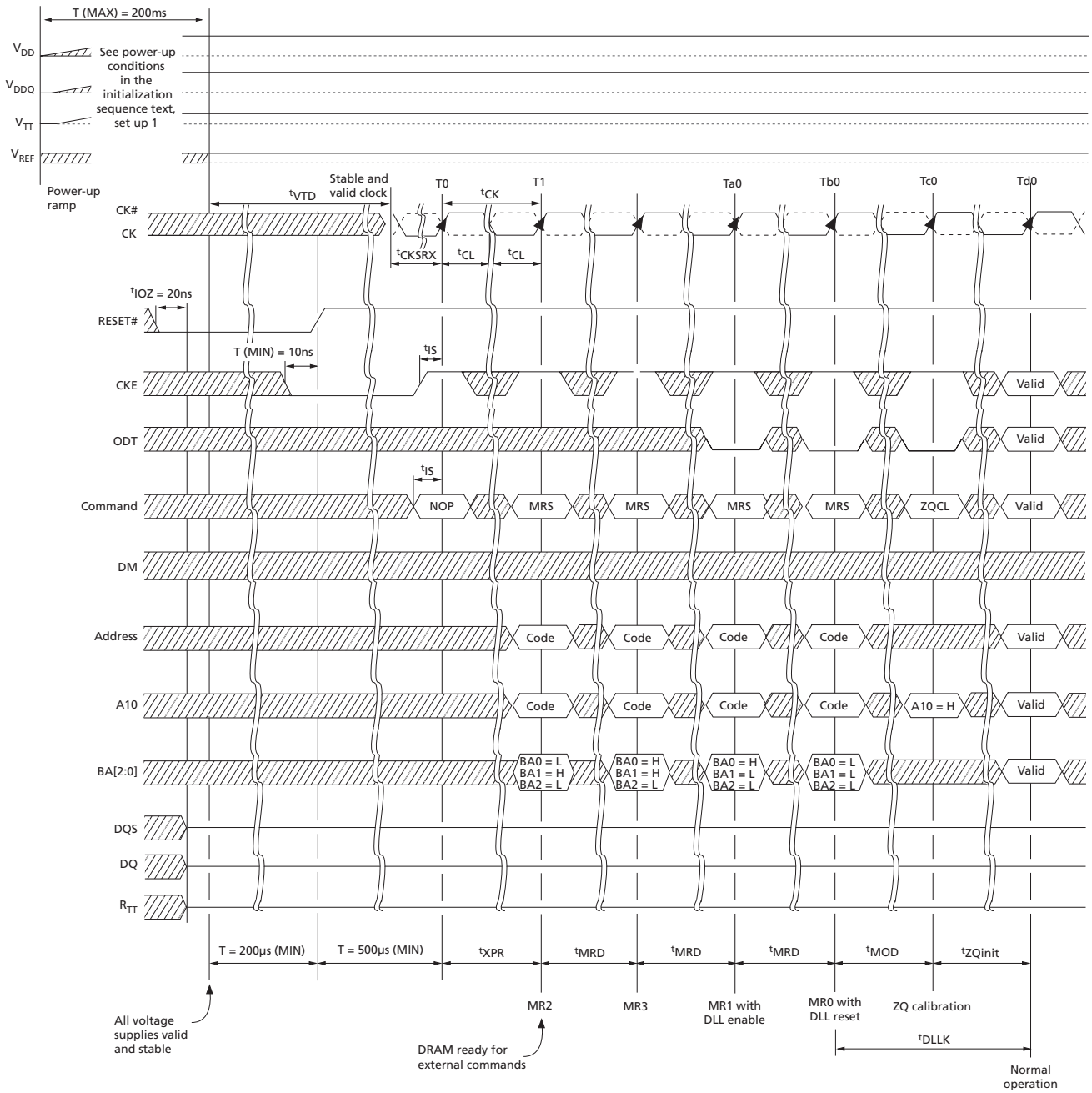
Figure 45: Initialization Sequence
