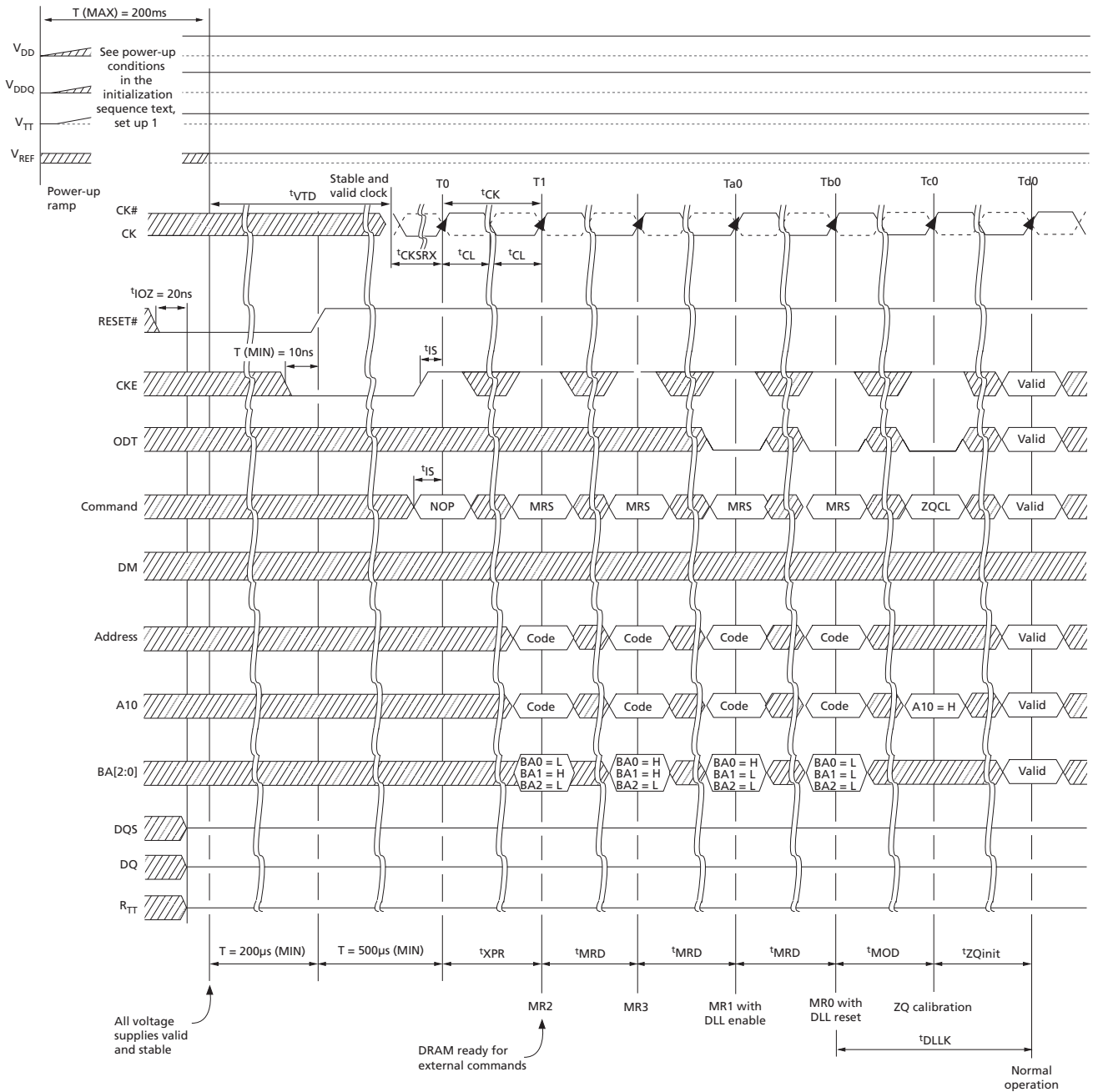
Figure 45: Initialization Sequence
