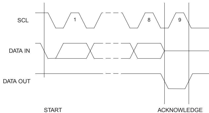
Figure 4-5. Output Acknowledge
