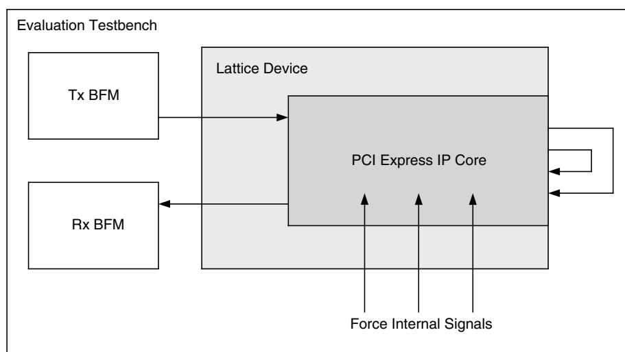
Figure 5-1. PCI Express RC-Lite IP Core Evaluation Testbench Block Diagram
