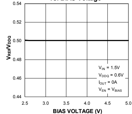
V_{REF}/V_{DDQ} Tracking Ratio vs. BIAS Voltage
