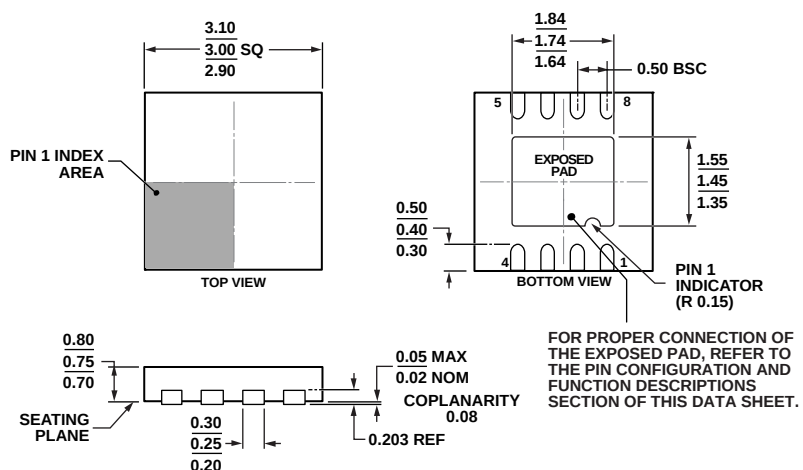
Figure 27. 8-Lead Lead Frame Chip Scale Package [LFCSF_WD] 3 mm × 3 mm Body, Very Very Thin, Dual Lead (CP-8-13)
