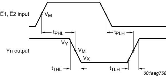
Fig. 7. Input (E1, E2) to output (Yn) propagation delays and output transition times
