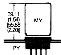
Mounting height of relay with socket
