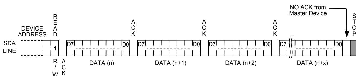
Figure 18 Sequential Read
