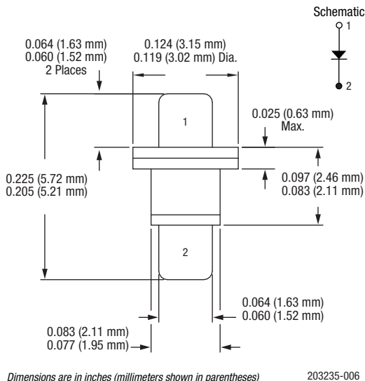
Figure 6. -210 Package
