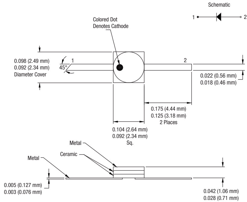
Figure 8. -240 Package
