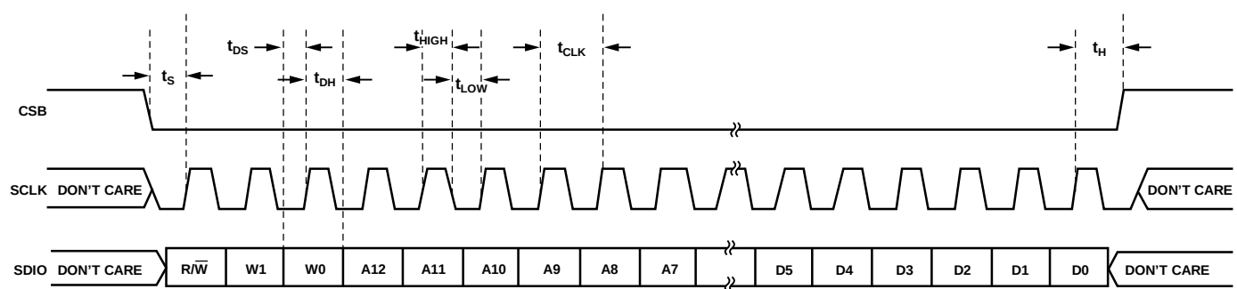
Figure 84. Serial Port Interface Timing Diagram
