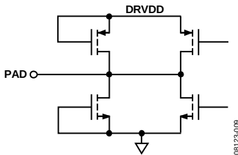
Figure 57. Digital Output
