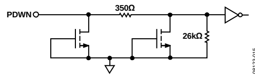
Figure 63. Equivalent PDWN Input Circuit
