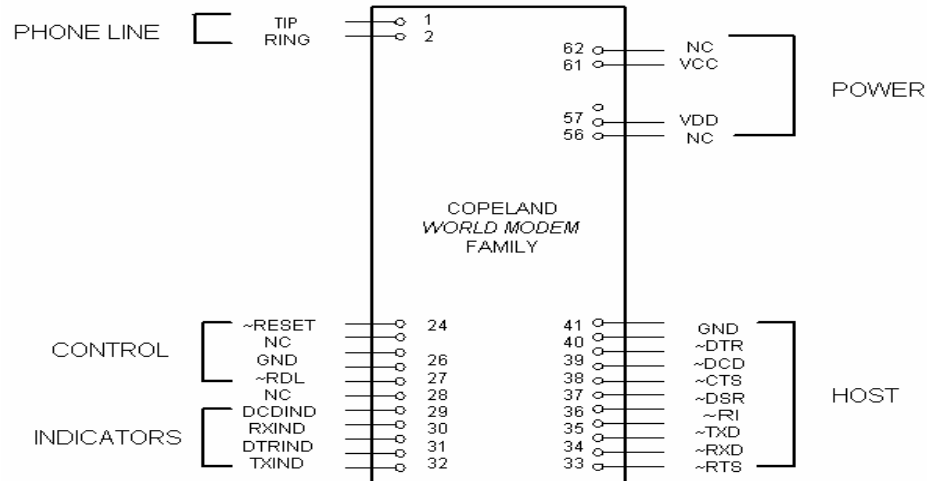
Serial Host Interface
