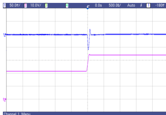
Fig. 35 AVO50-48S2V5 typical transient response to step increase in load from 50% to 75% of full load, room temperature, 48Vdc input ( \Delta I_o/\Delta t = 0.1A/1\mu s )
