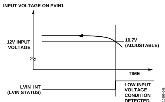
Figure 55. Low Input Voltage Warning Function ( V_{IN} = 12\text{ V} )
