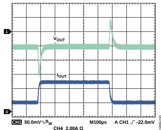
Figure 32. Channel 1/Channel 2 Load Transient, 1 A to 4 A, V_{IN} = 12\text{ V} , V_{OUT} = 3.3\text{ V} , f_{SW} = 600\text{ kHz} , L = 2.2\text{ }\mu\text{H} , C_{OUT} = 47\text{ }\mu\text{F} \times 2
