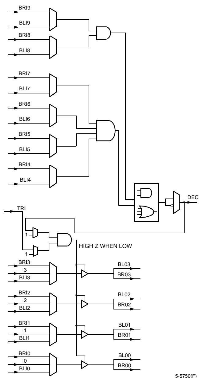
Figure 15. Buffer-Decoder-Decoder Mode
