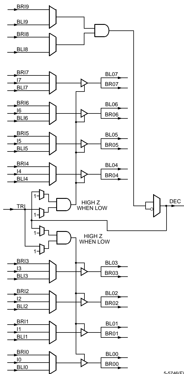
Figure 13. Buffer-Buffer-Decoder Mode
