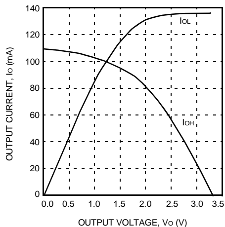
Figure 100. Fast ( T_J = 25^\circ\text{C} , V_{DD} = 3.3\text{ V} ) Lucent Technologies Inc.
