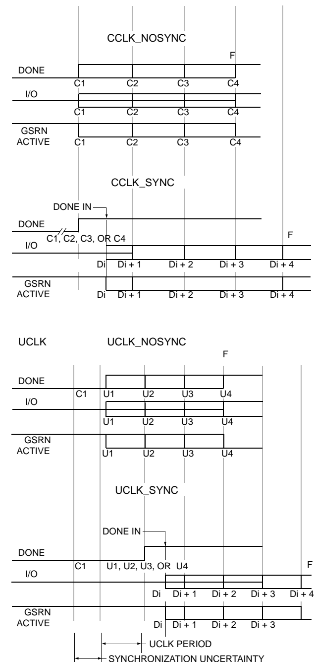
Figure 51. Start-Up Waveforms
