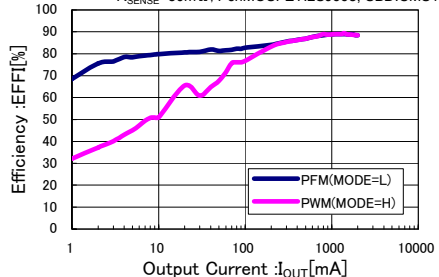
XC9252x08A ( V_{IN}=24V , V_{OUT}=12V , f_{OSC}=280kHz )
