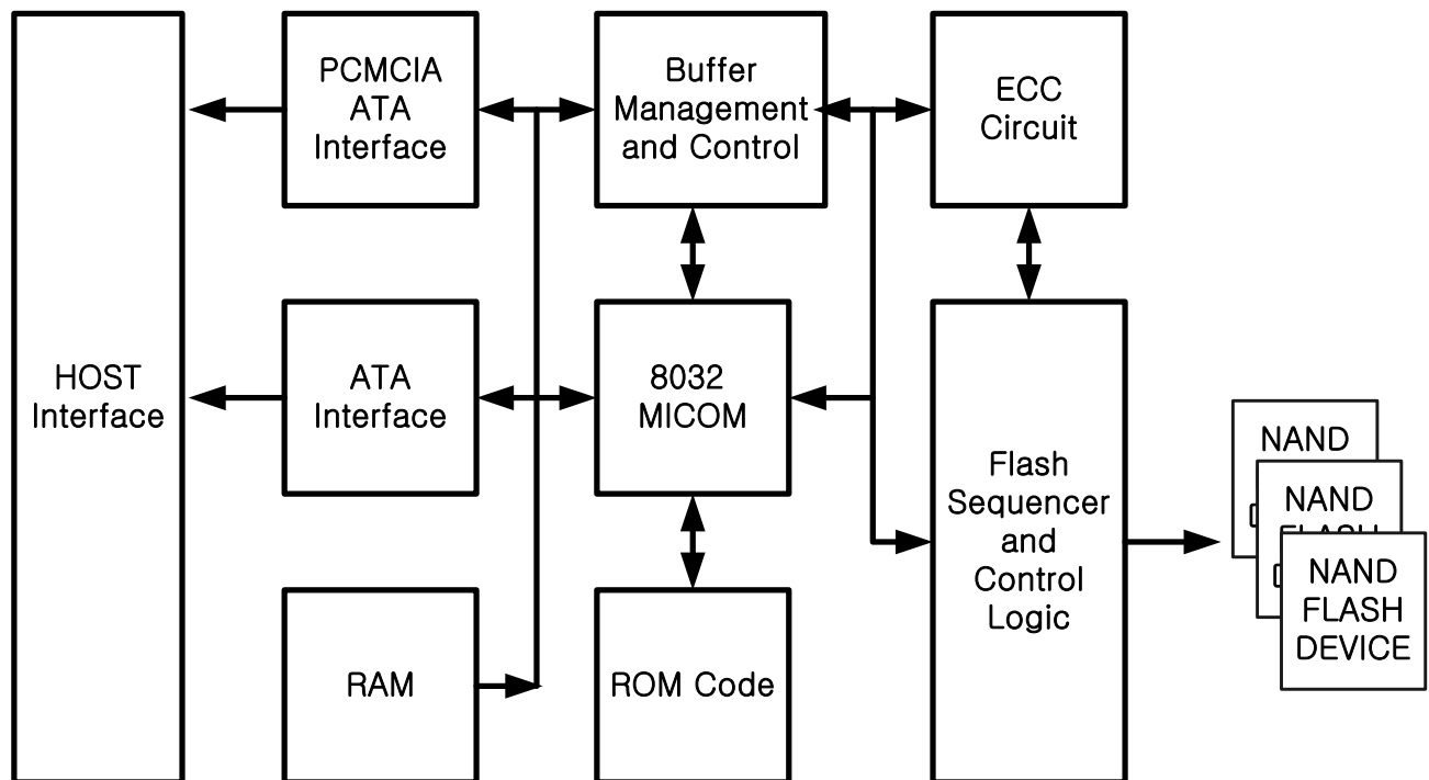
Figure 2.1 Block Diagram
