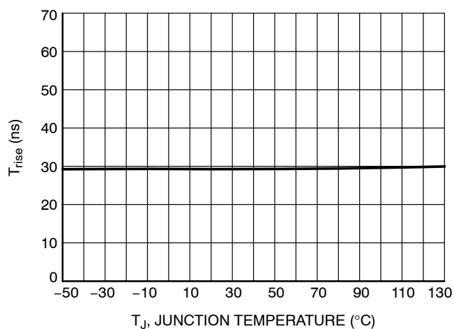
Figure 16. DRV Voltage Rise-Time ( C_L = 1 nF, 10–90% of Output Signal) vs. Temperature
