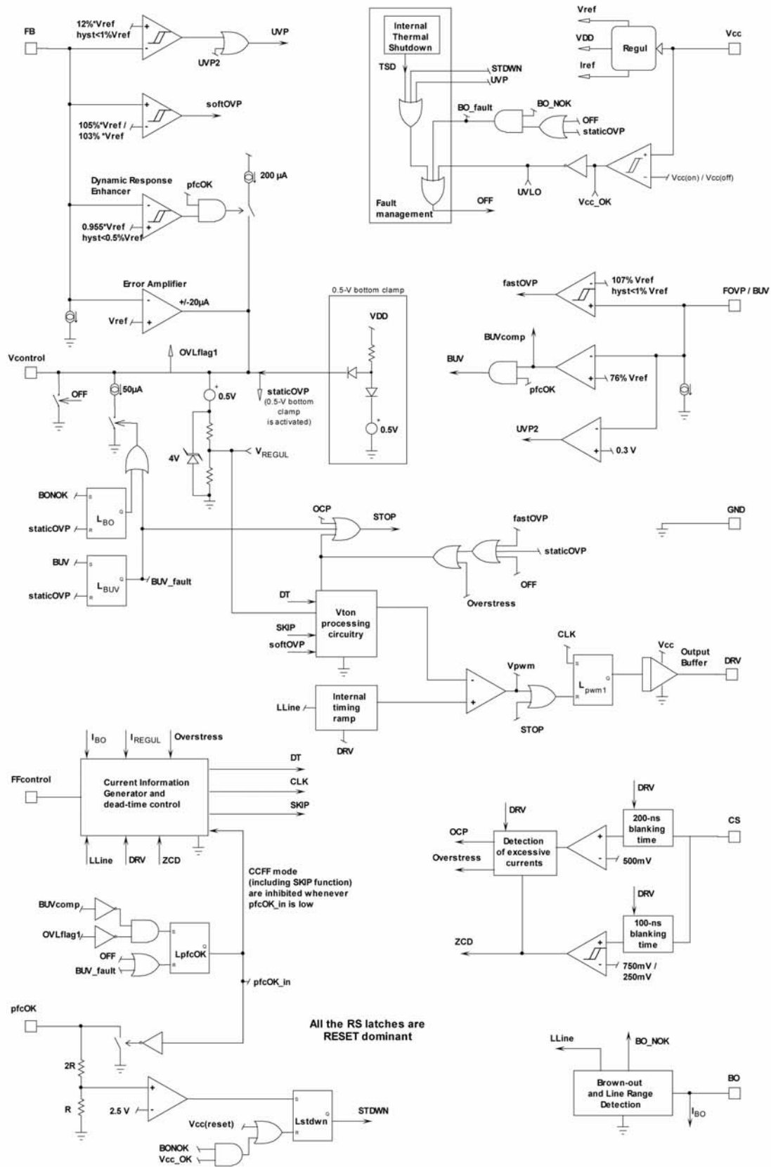
Figure 2. Block Diagram
