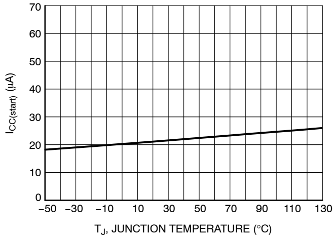
Figure 7. Start-Up Current @ V_{CC} = 9.4 V vs. Temperature
