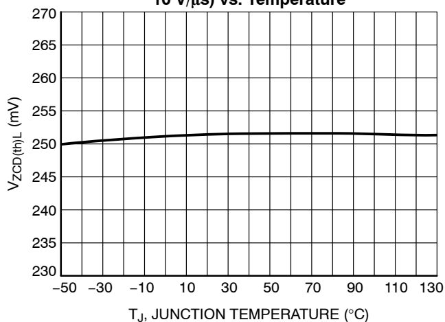
Figure 30. Zero Current Detection, V CS/ZCD Falling vs. Temperature
