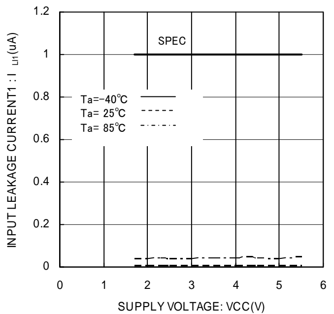
Figure 11. Input leakage current1 I_{IL1} (SK)
