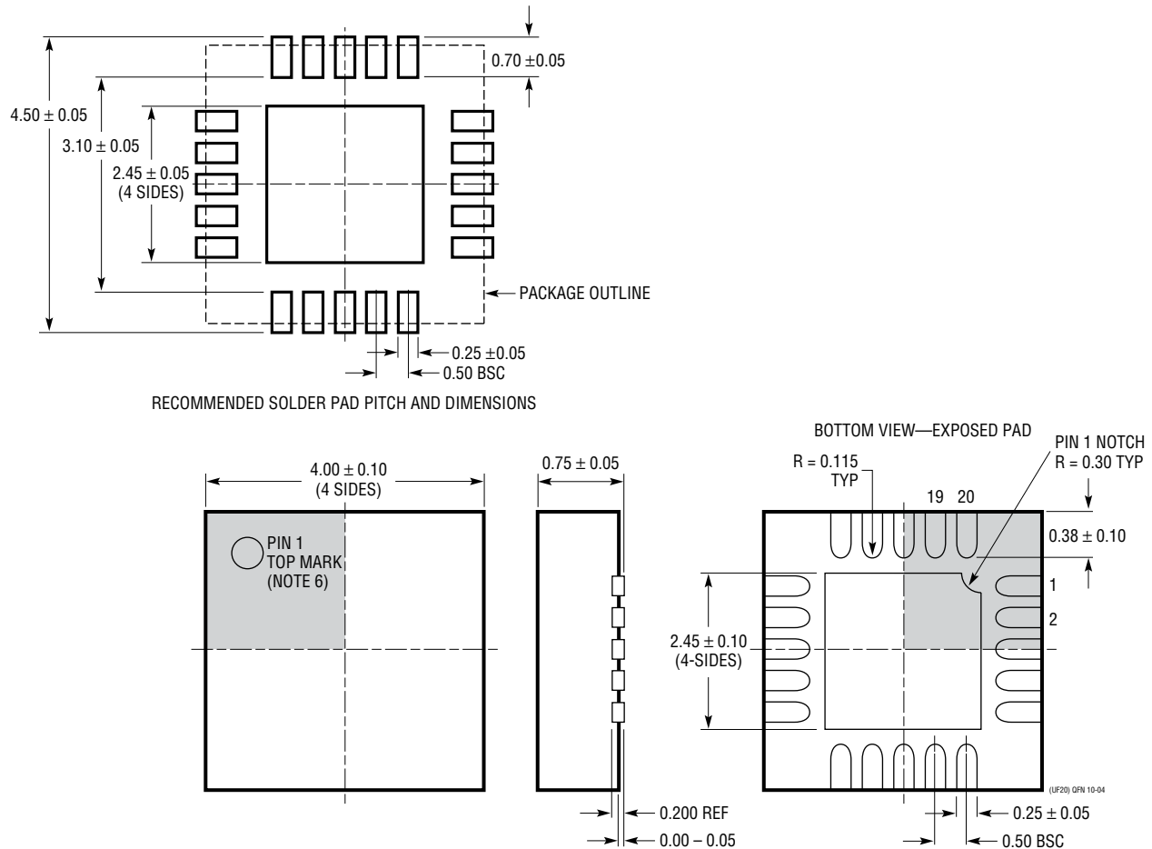
UF Package 20-Lead Plastic QFN (4mm × 4mm) (Reference LTC DWG # 05-08-1710)
