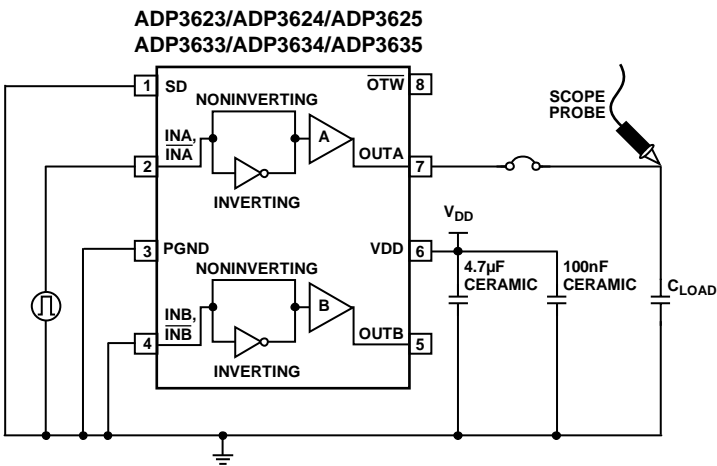
Figure 20. Test Circuit
