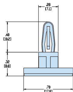
BAYONET SNAP LOCK 10,2 / ADHESIVE-BACK BASE 17,8 sq
